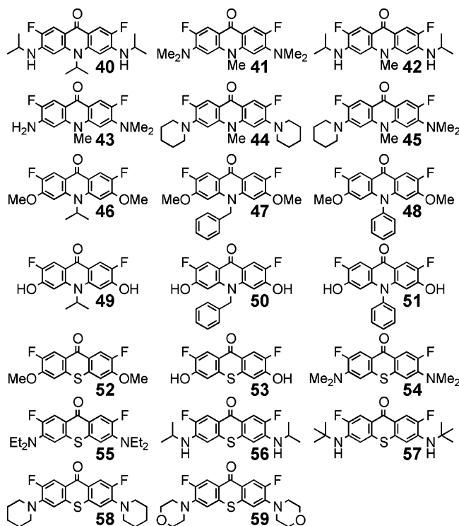
Figure 3. Structures of fluorinated acridones and thioxanthenone products.
