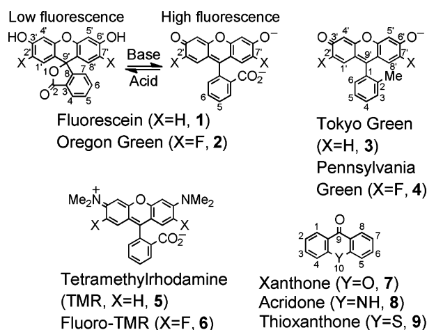
Figure 1. Structures of fluorinated fluorophores and related compounds.
